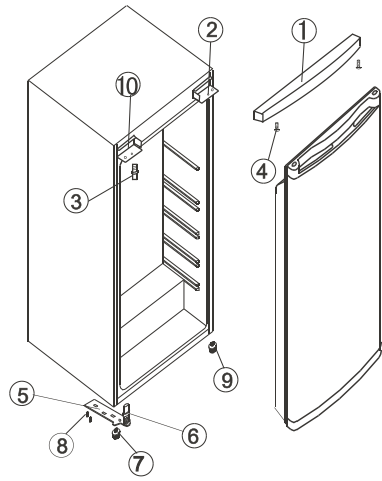
FIGURE 1 - REPRESENTS POSITION OF COMPONENTS PRIOR TO DOOR REVERSAL.
