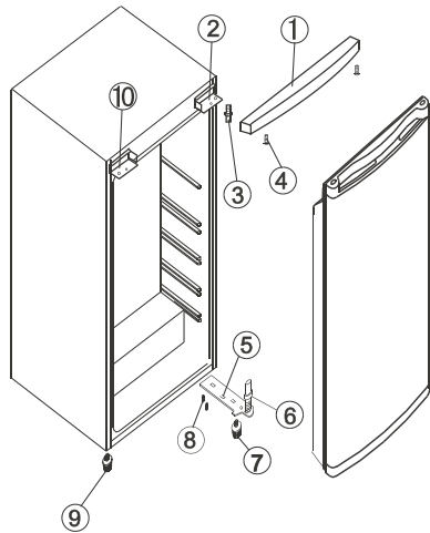
FIGURE 1 - REPRESENTS POSITION OF COMPONENTS PRIOR TO DOOR REVERSAL.
